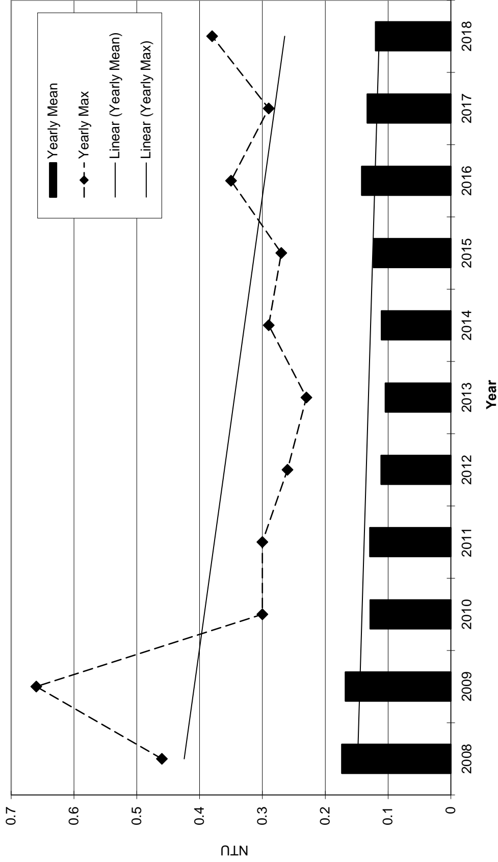
Figure 8.1: Yearly Mean and Max Turbidity Results for Round Hill General Improvement District between July 1, 2008 and June 30, 2019.
