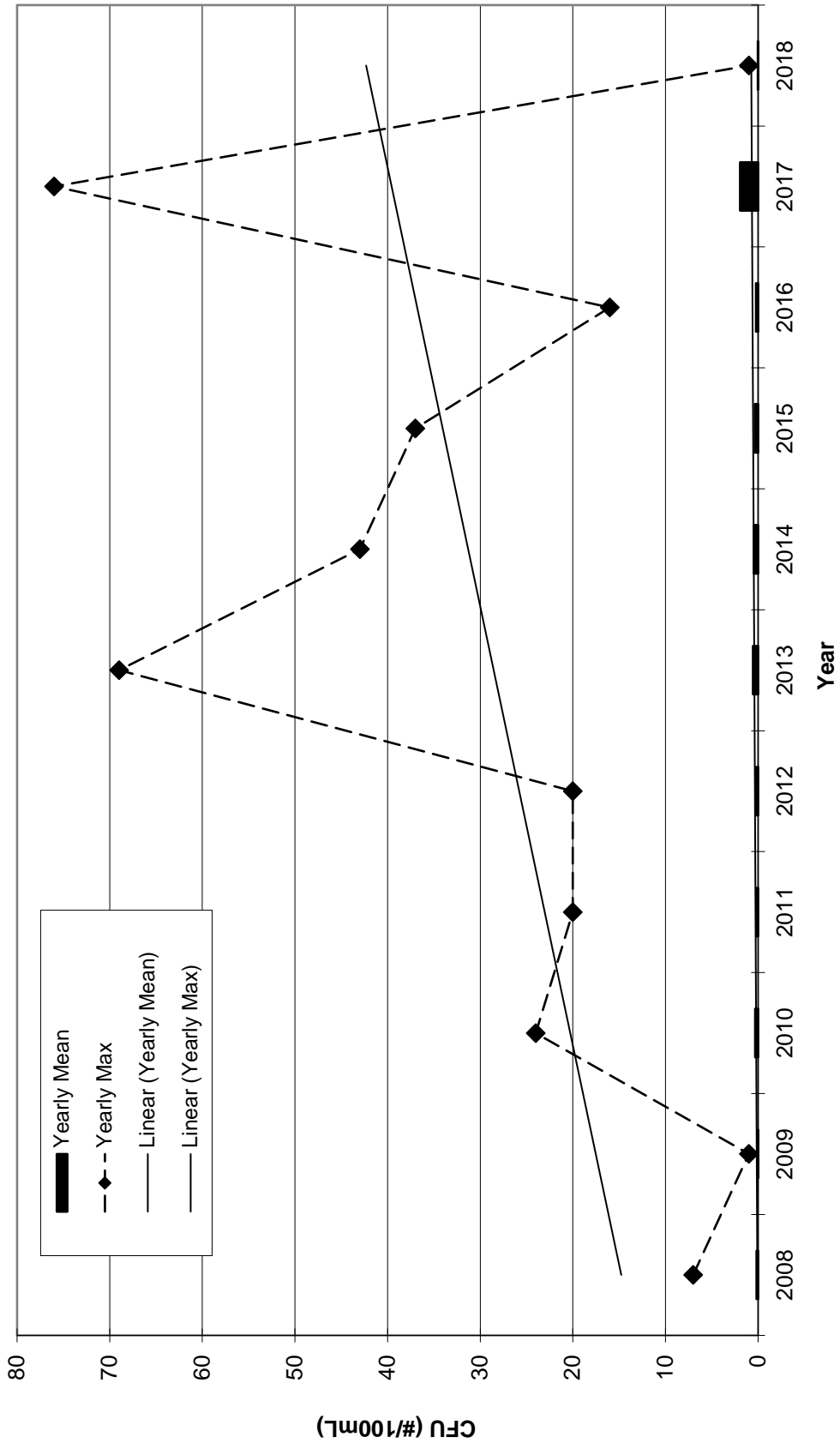
Figure 5.3: Yearly Mean and Max Coliform Results for Incline Village General Improvement District between July 1, 2008 and June 30, 2019.
