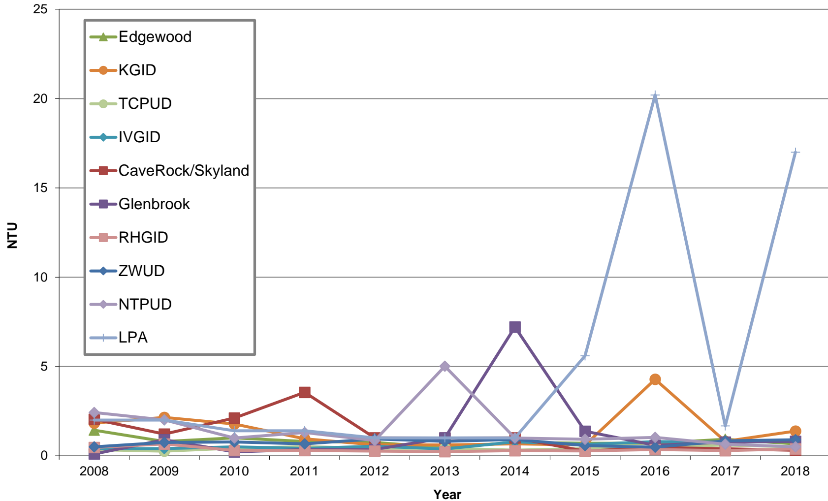
Figure 1.1: Comparison of TWSA Purveyors Maximum Turbidity Results from 2008 to 2019.
