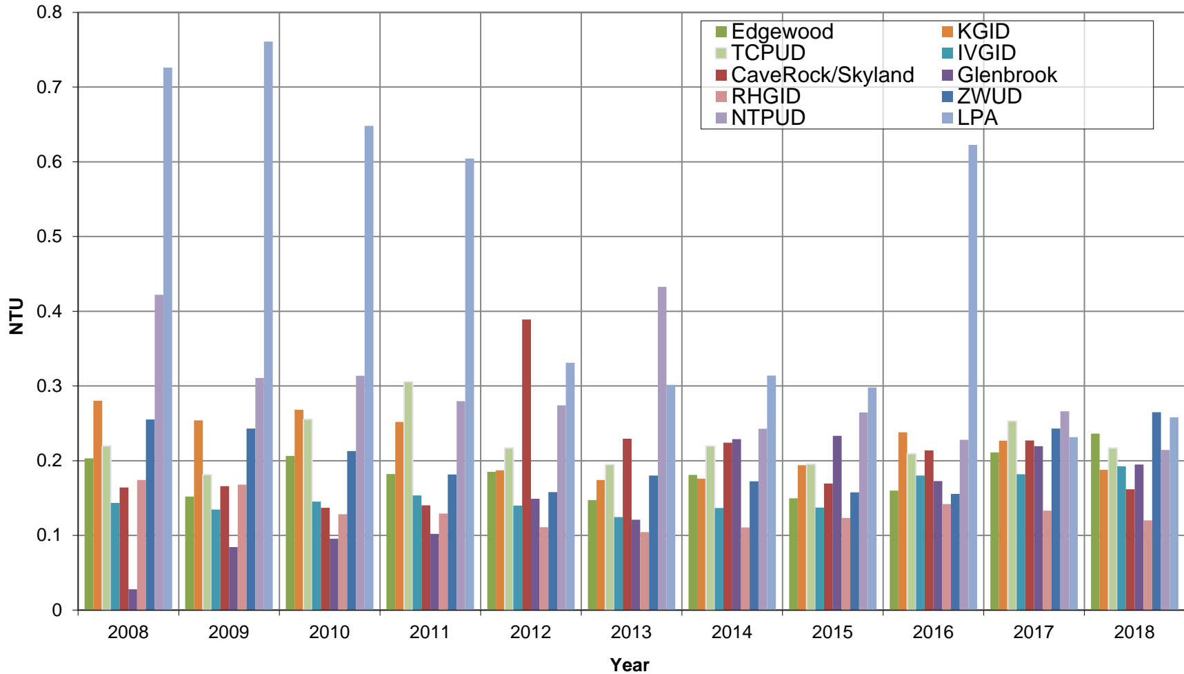
Figure 1.2: Comparison of TWSA Purveyors Annual Mean Turbidity for the 2008-2019 Reporting Years.
