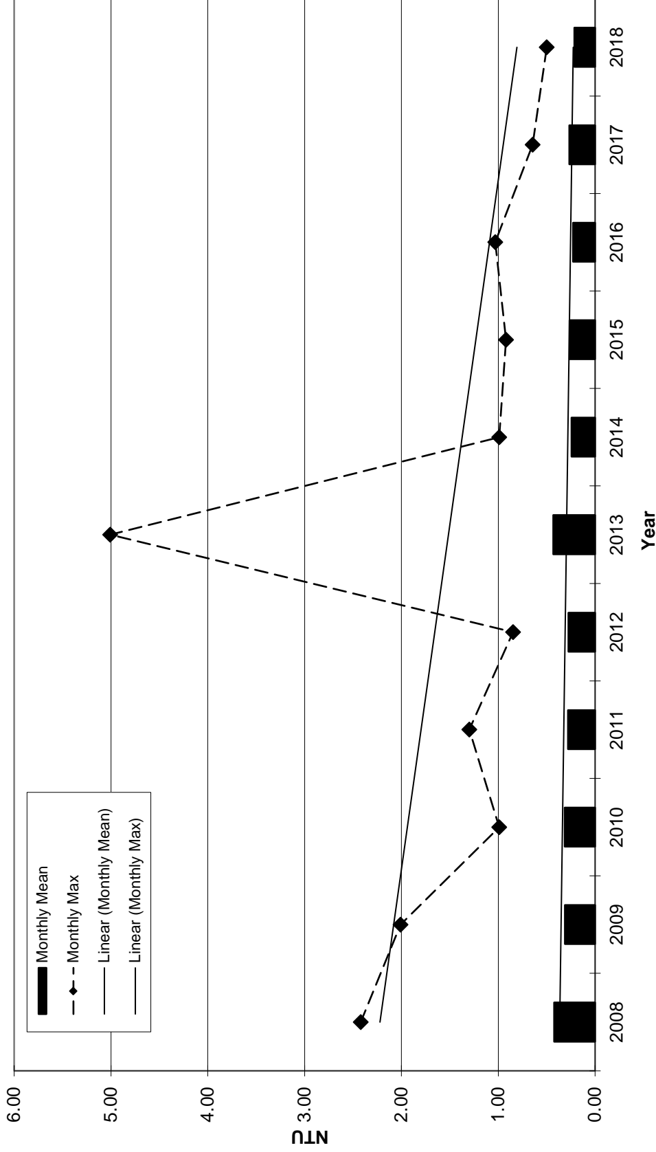
Figure 10.1: Yearly Mean and Max Turbidity Results for North Tahoe Public Utility District between July 1, 2008 and June 30, 2019.
