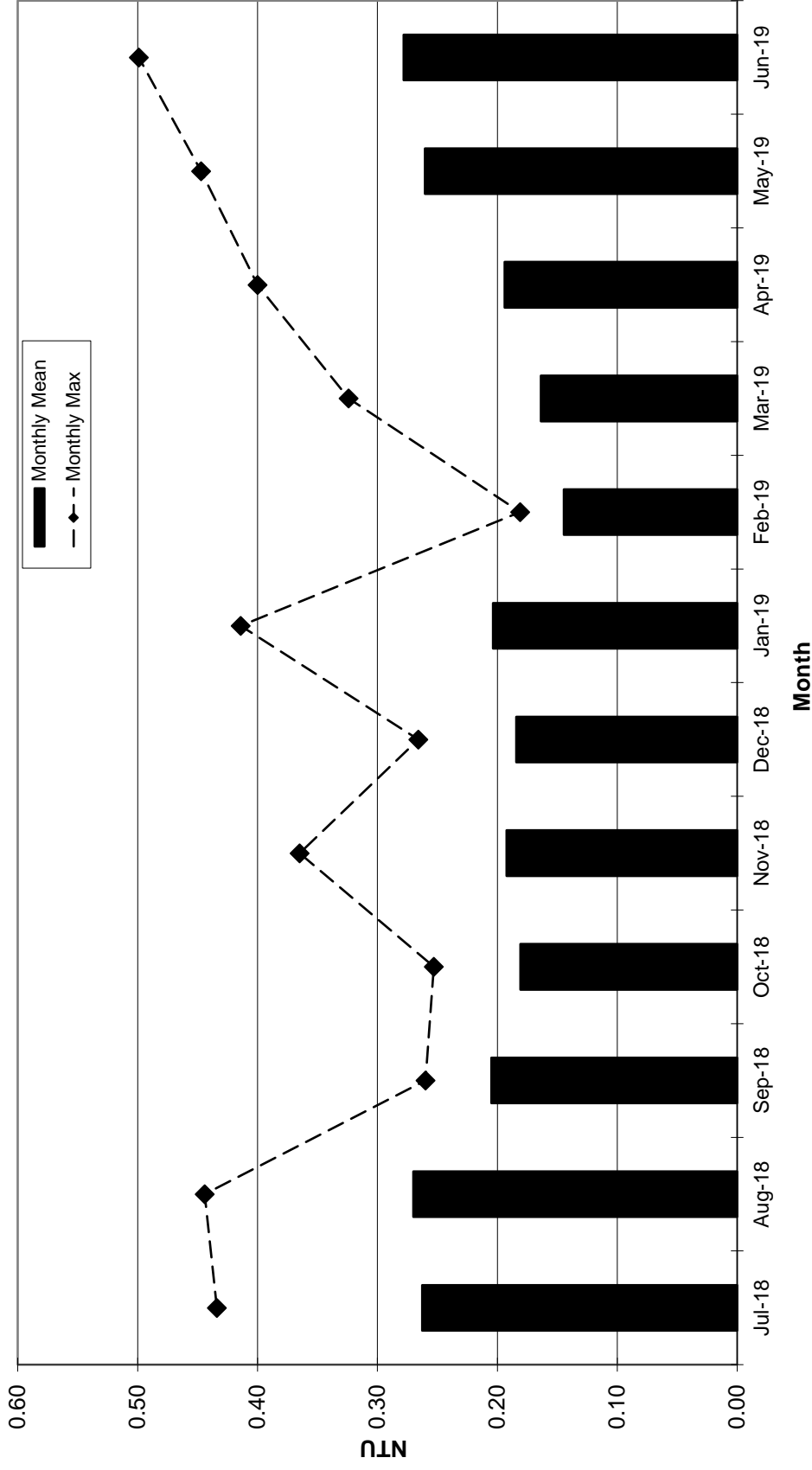
Figure 10.0: Monthly Mean and Max Turbidity Results for North Tahoe Public Utility District between July 1, 2018 and June 30, 2019.
