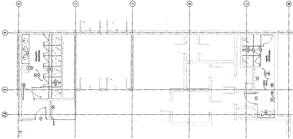
UPPER LEVEL DEMO PLAN 0' 0" to 0' 6" = 1/8" = 1'-0"
