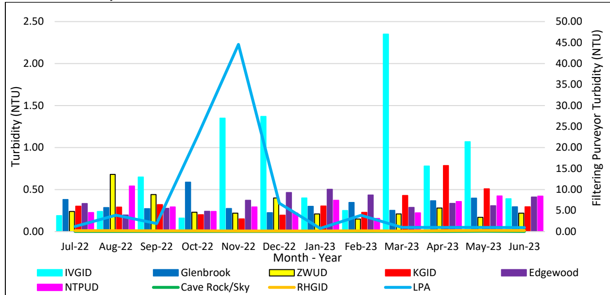
Figure 1.1: Maximum turbidity from July 1, 2022 to June 30, 2023. Purveyors operating with filtration avoidance are represented by bars on the primary axis, and filtering purveyors are represented by lines on secondary access.
