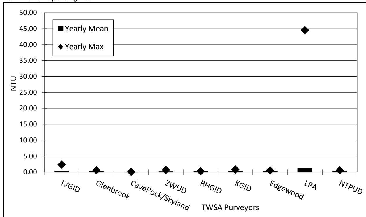
Figure 1.0: Comparison of Annual Mean and Maximum Turbidity Results for TWSA Purveyors for the 2022-2023 Reporting Year.
