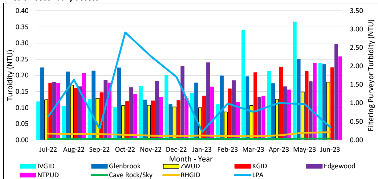
Figure 1.2: Mean turbidity by month July 2022 to June 2023. Purveyors operating with filtration avoidance are represented by bars on the primary axis, and filtering purveyors are represented by lines on secondary access.
